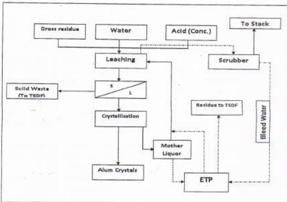
Figure no.: 1-Process flow diagram for utilization of hazardous waste i.e., Aluminium dross residues.
